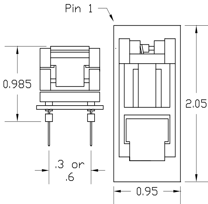
PA5114-20SO
